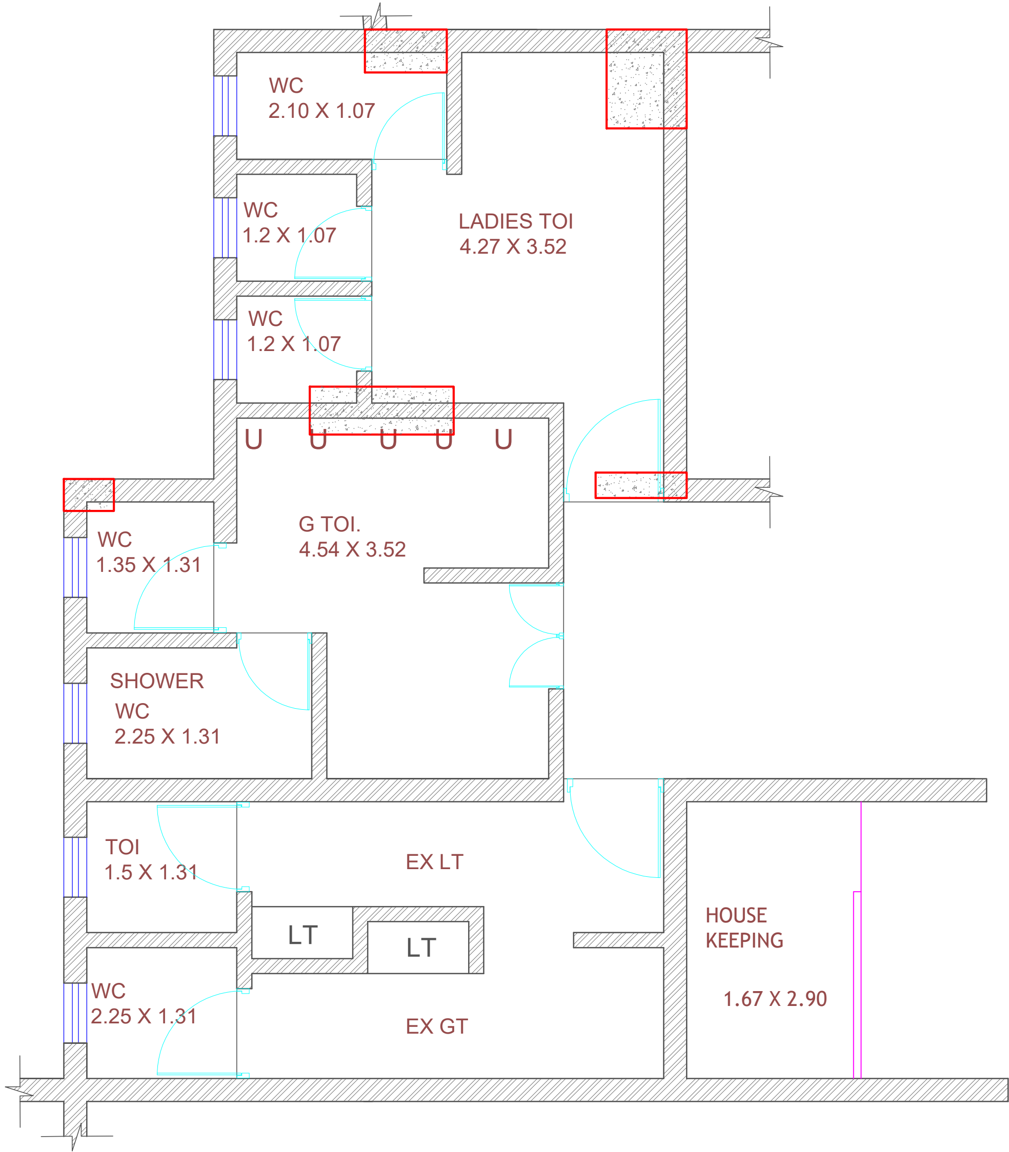
Second & Third floor Existing washroom layout
