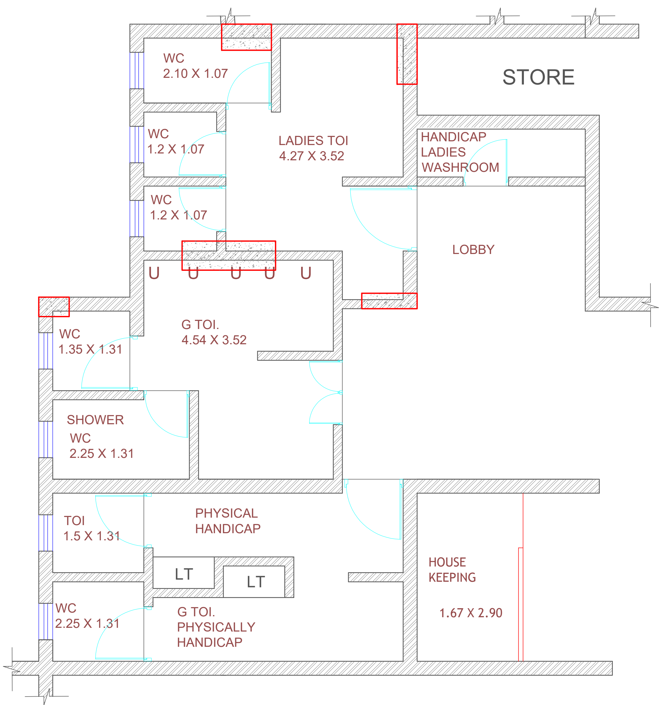
Ground floor Existing washroom layout
