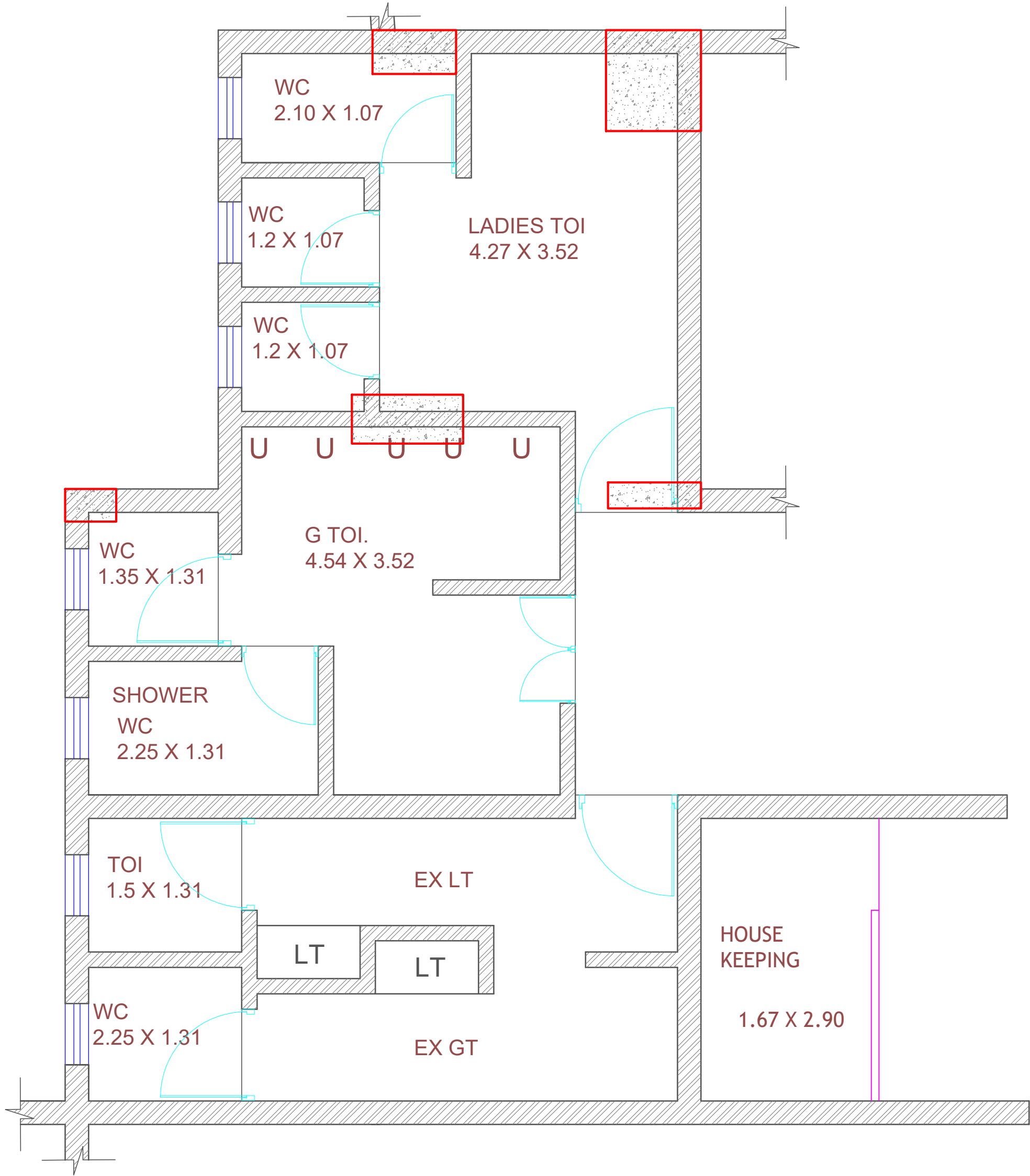
Fourth floor Existing washroom layout
